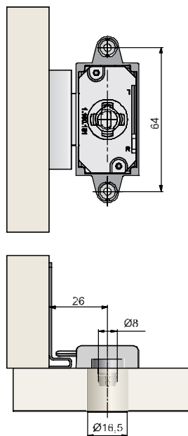
Type 539 dübelbar / to fasten with dowels
