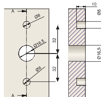
Bohrbild Drilling template
