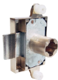
Type 539 Kastenschloss dübelbar case lock with dowels
