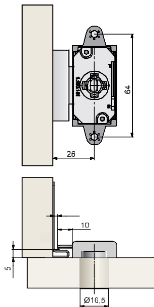
Type 530 schraubbar / screw fixing
