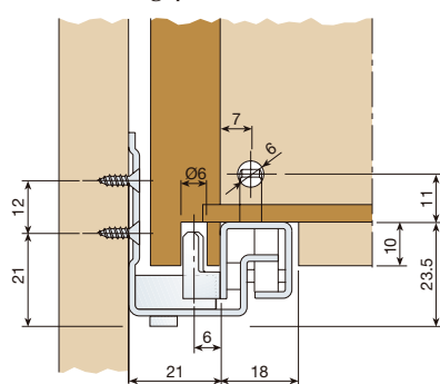
Drilling pattern
