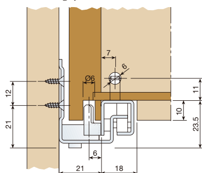
Drilling pattern
