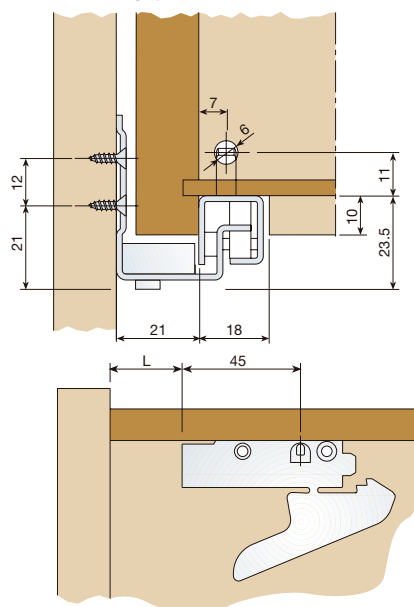
Drilling pattern
