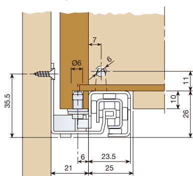
Drilling Pattern
